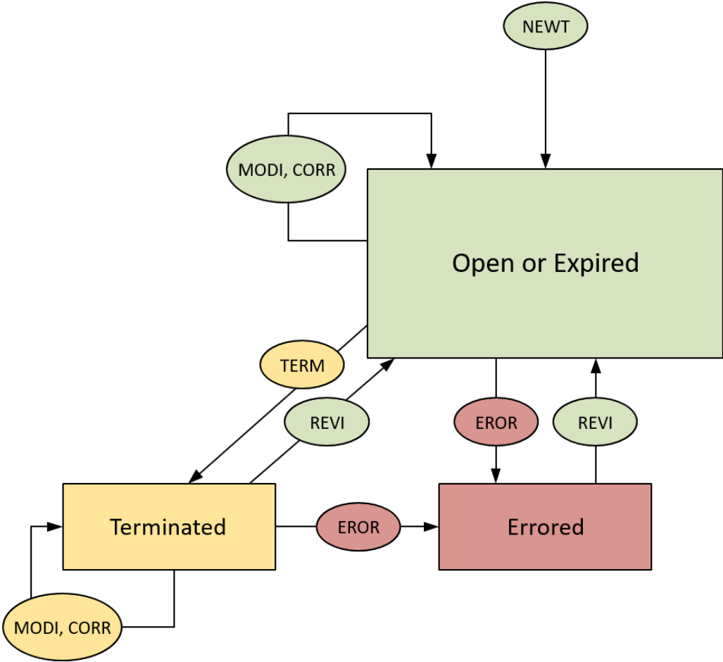
Figure 2 - Permitted Action type sequences for Part 43 Reporting
